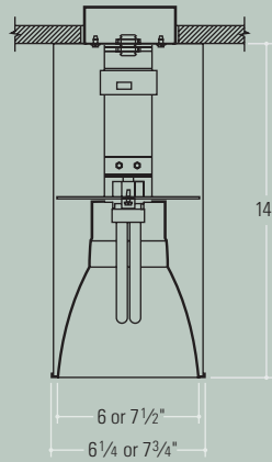
SURFACE MOUNT
