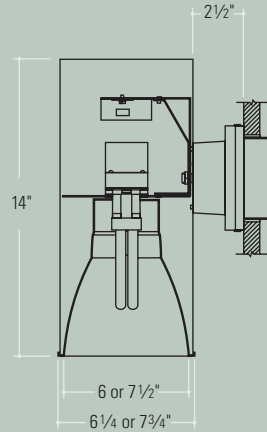
WALL MOUNT
